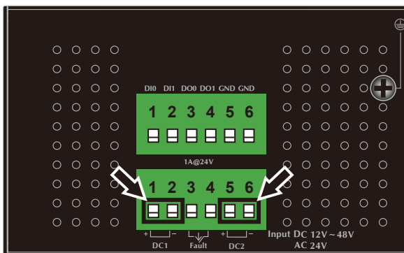
Figure 3-2: IGS-6325-8T4X/IGS-6325-8T8S4X Upper Panel
