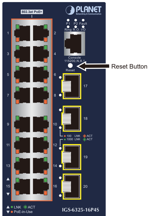
Figure 6-1: IGS-6325 Series Reset Button
